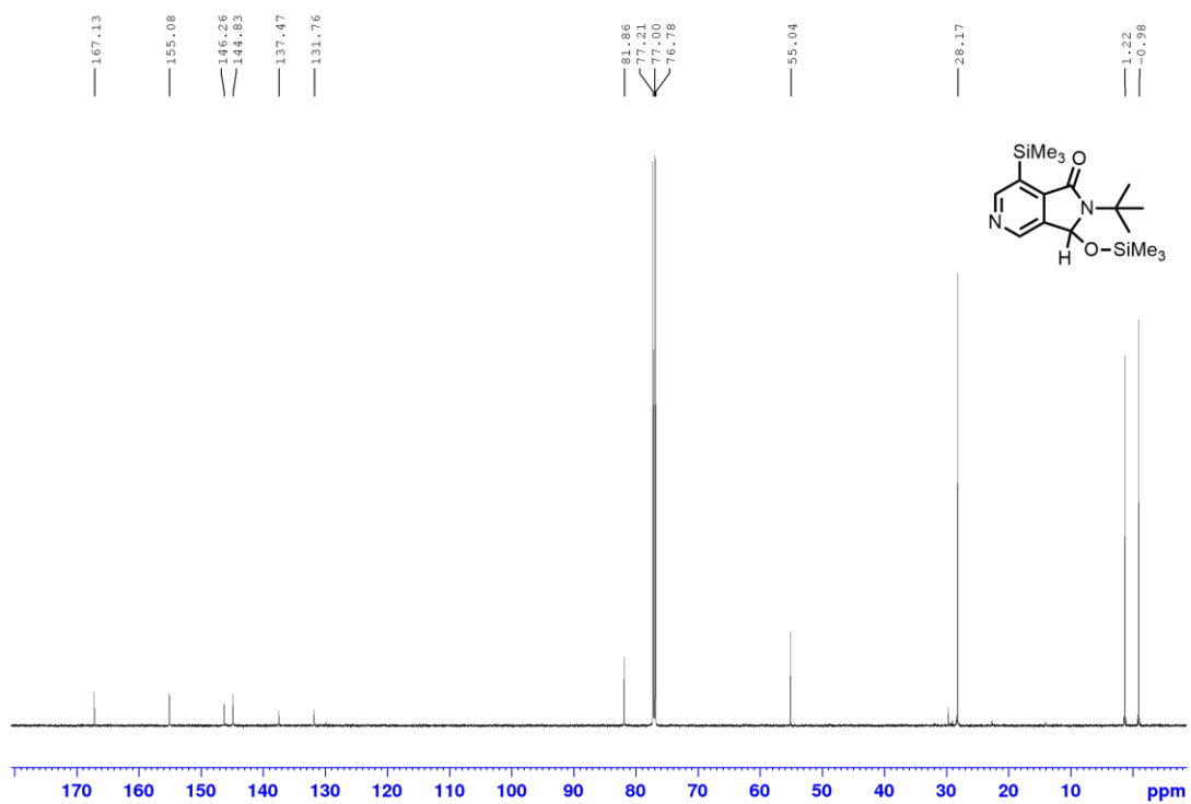
Figure S2. ^{13}\text{C} NMR spectrum of compound 3b (150 MHz, \text{CDCl}_3 , room temperature).
