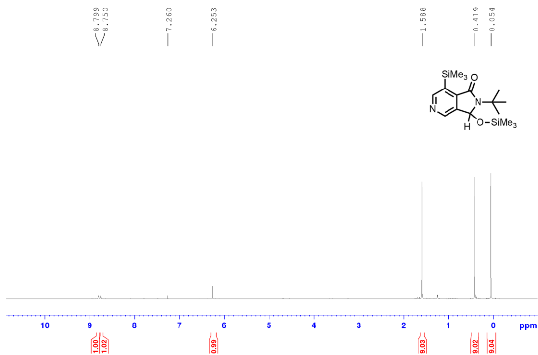
Figure S1. 1 H NMR spectrum of compound 3b (600 MHz, CDCl 3 , room temperature).
